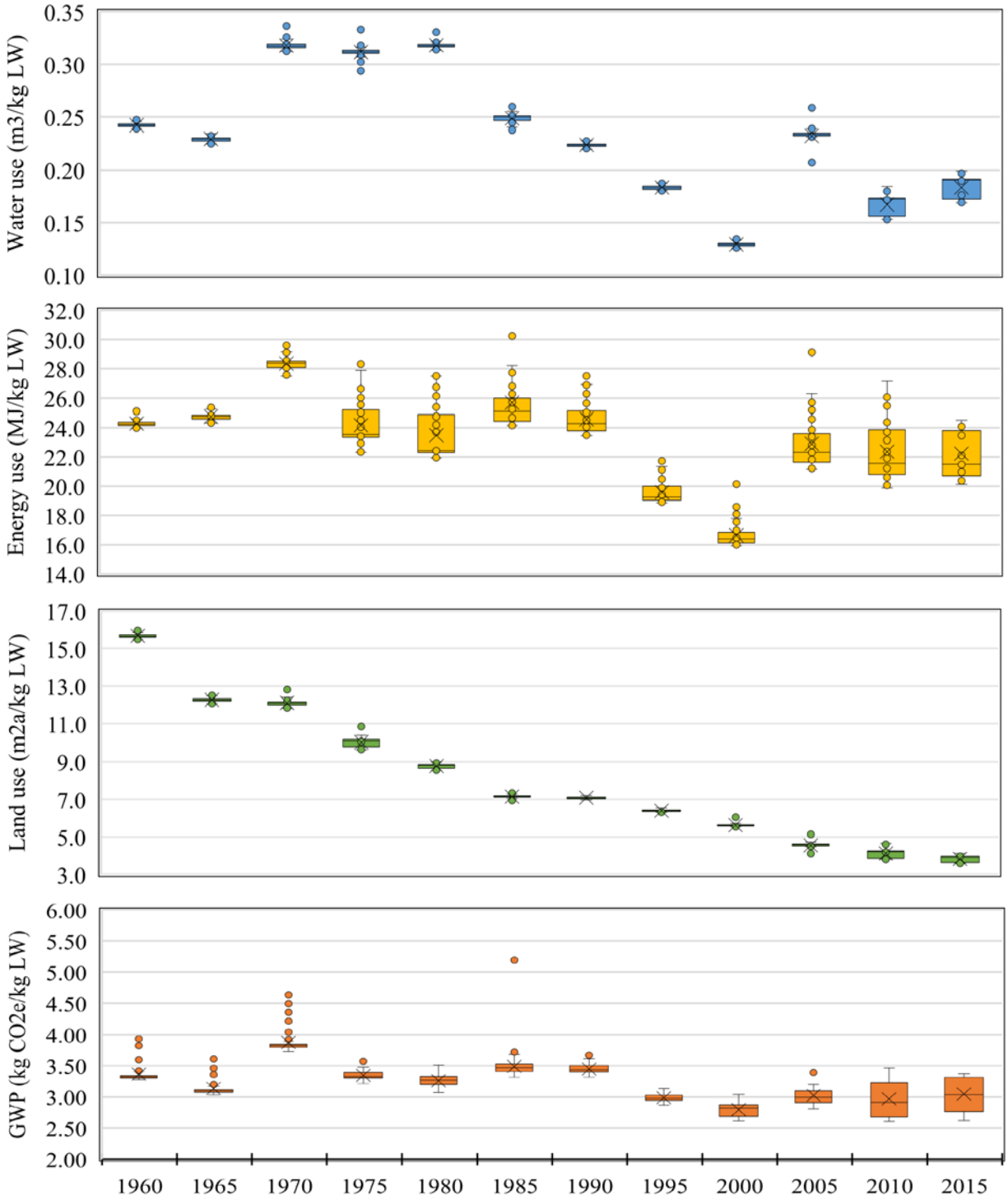
Figure 7. LCIA results for all the simulated counties. Boxes represent 50 percent of simulated counties, with the center line representing the median and the X representing the mean. Whiskers are the expected minimum and maximum values. Circles represent outliers, defined as being more than 1.5 times the interquartile range (size of the box) above or below the box
