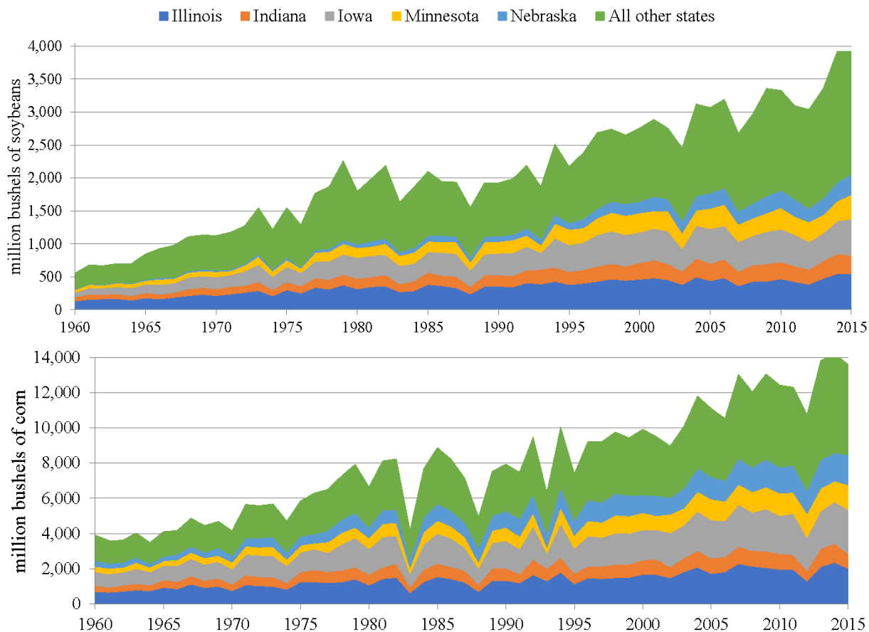
Figure 6. Corn and soybean production over the assessment period from the five states from which data were used to inform the corn and soybean LCI processes along with production from the rest of the United States.
