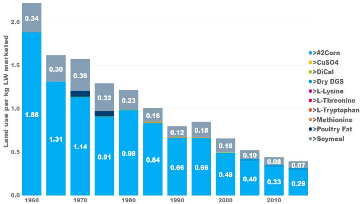
Figure 23. Land use associated with production the sow barn ration for 1 kg LW marketed.
